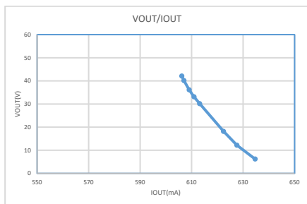
Operating Window
