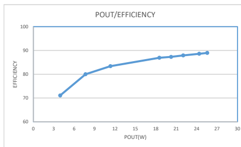
Efficiency Vs Output Power
