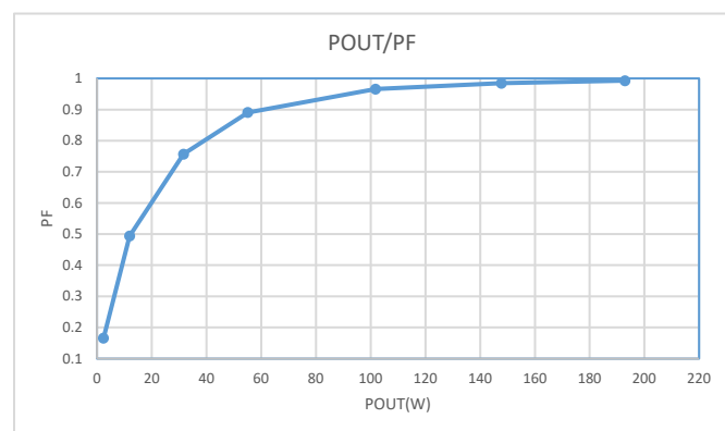
Power Factor Vs Output Power
