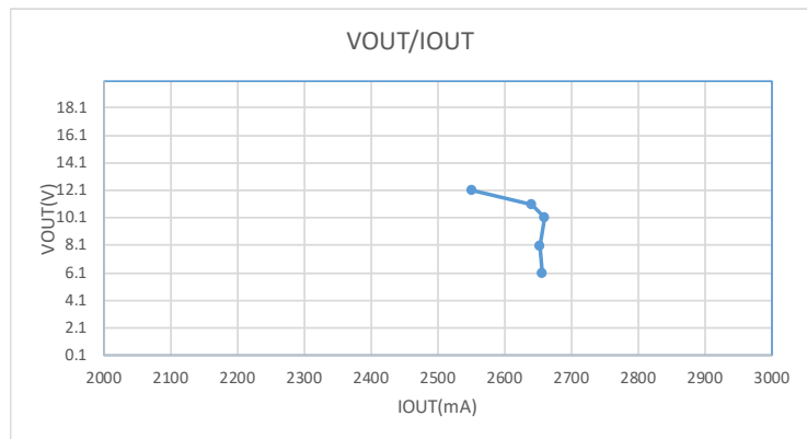
Operating Window (CC)
