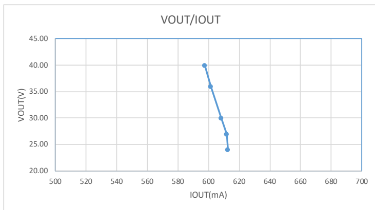
Operating Window
